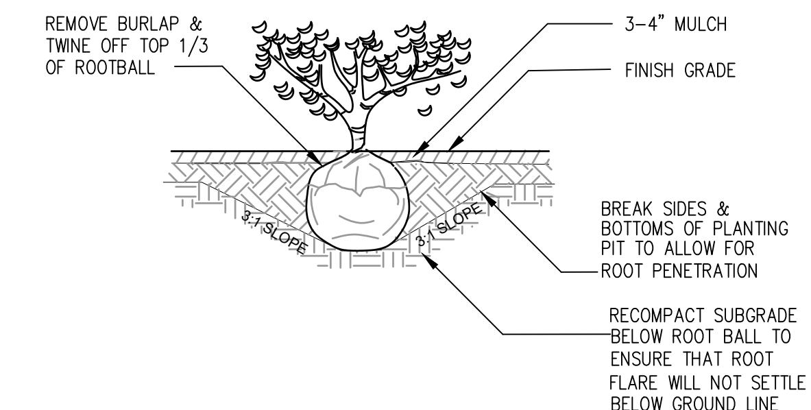
4 TYPICAL SHRUB PLANTING DETAIL NTS
